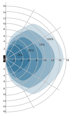
Wall mounting pattern (Unit: m)
